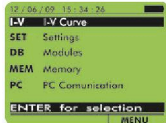
General menu
