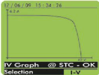
I-V curve
