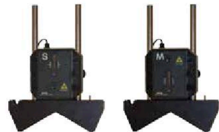
The alignment sensors are identical with exception of the position of laser diode and the knob for adjustment of the laser on the 'M' sensor. Sensor size: 86x81,5x36 mm, weight: 230 g
